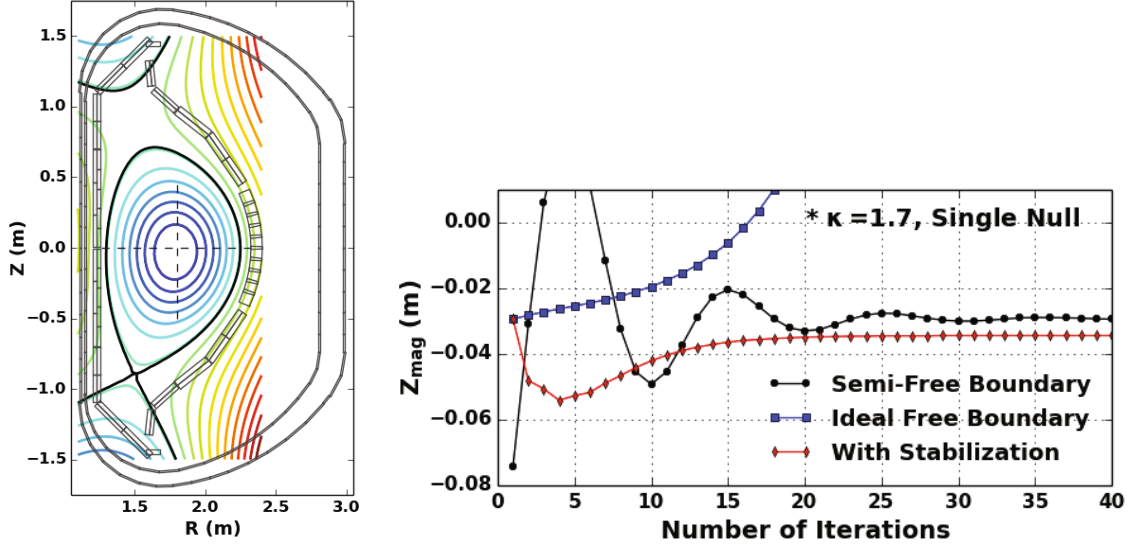
Fig. 5. (Color online) Vertical displacement responses to an initial perturbation of \Delta Z = -0.03 m are compared for the equilibrium shown on the left. The first one (black) is during TES iteration as a semi-free boundary problem, the second one (blue) as an ideally-free boundary problem, and the third one (red) with the generalized vertical stabilization.
